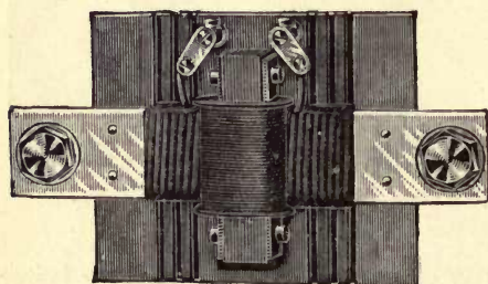
Fig. 141.—Current Transformer for 600 Amps
